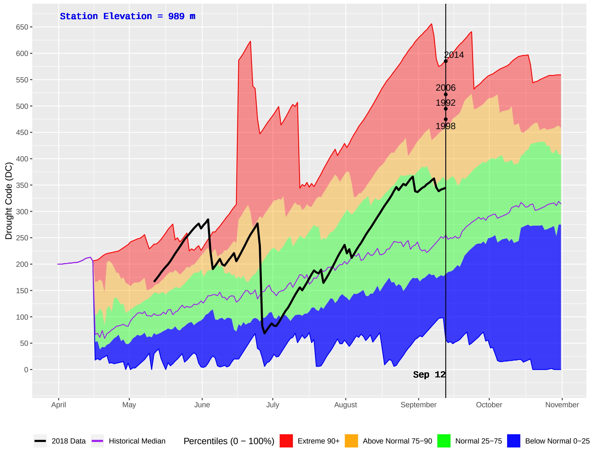
PINK MOUNTAIN (129) : Historical (1983–2016) and Current (2018) Daily Drought Code (DC)
