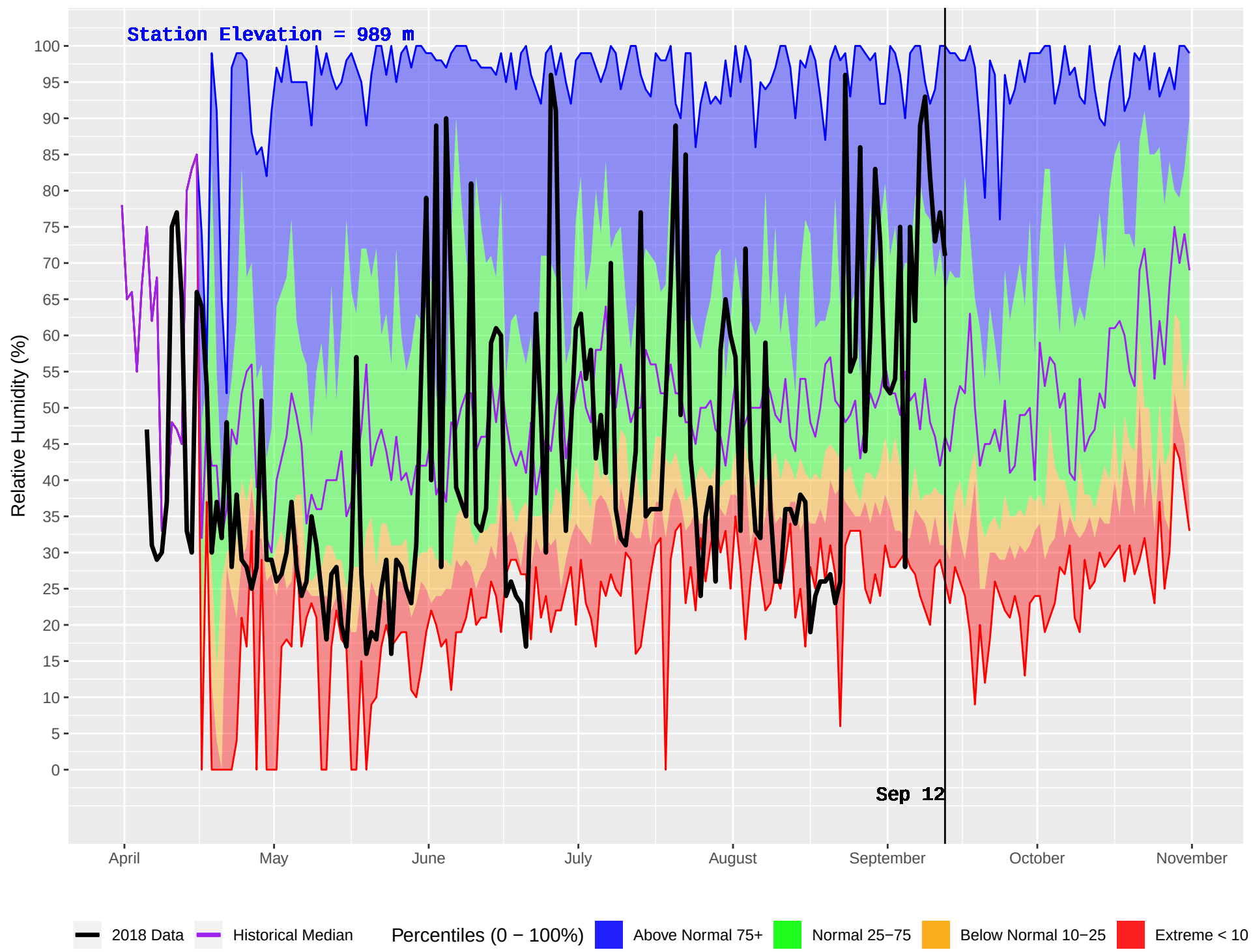
PINK MOUNTAIN (129) : Historical (1983–2016) and Current (2018) Daily Relative Humidity
