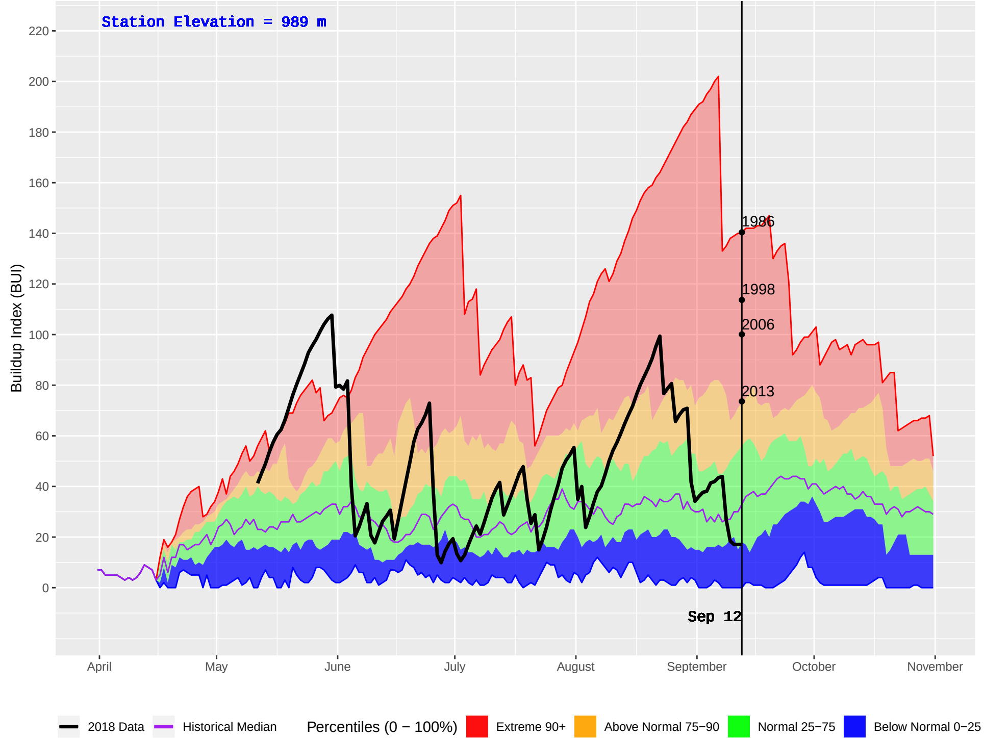
PINK MOUNTAIN (129) : Historical (1983–2016) and Current (2018) Daily Buildup Index (BUI)
