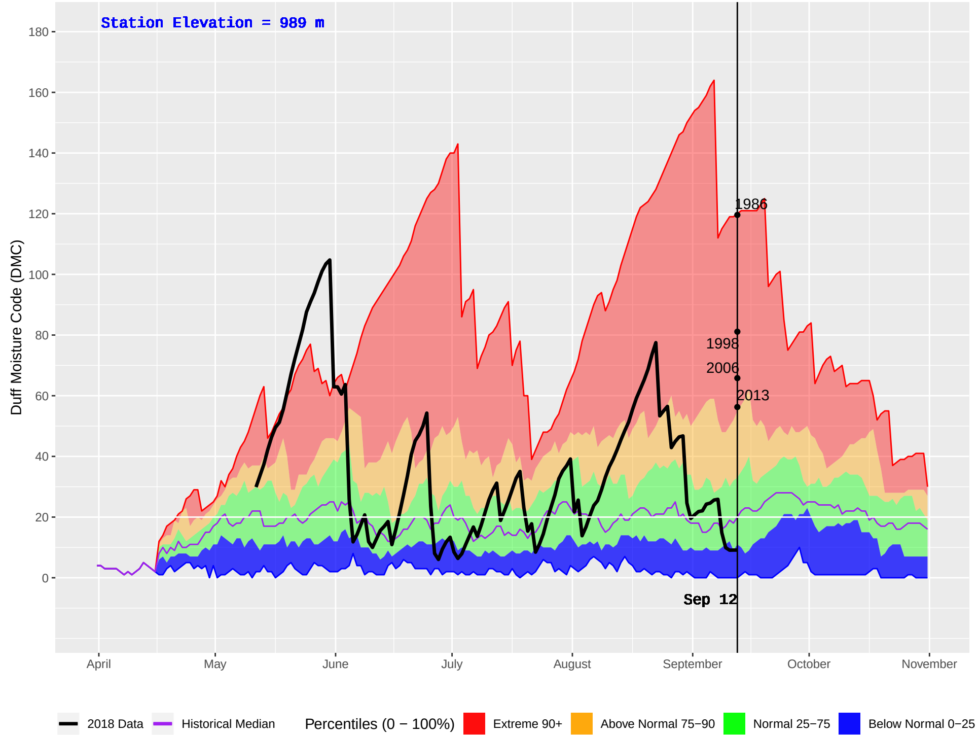
PINK MOUNTAIN (129) : Historical (1983–2016) and Current (2018) Daily Duff Moisture Code (DMC)
