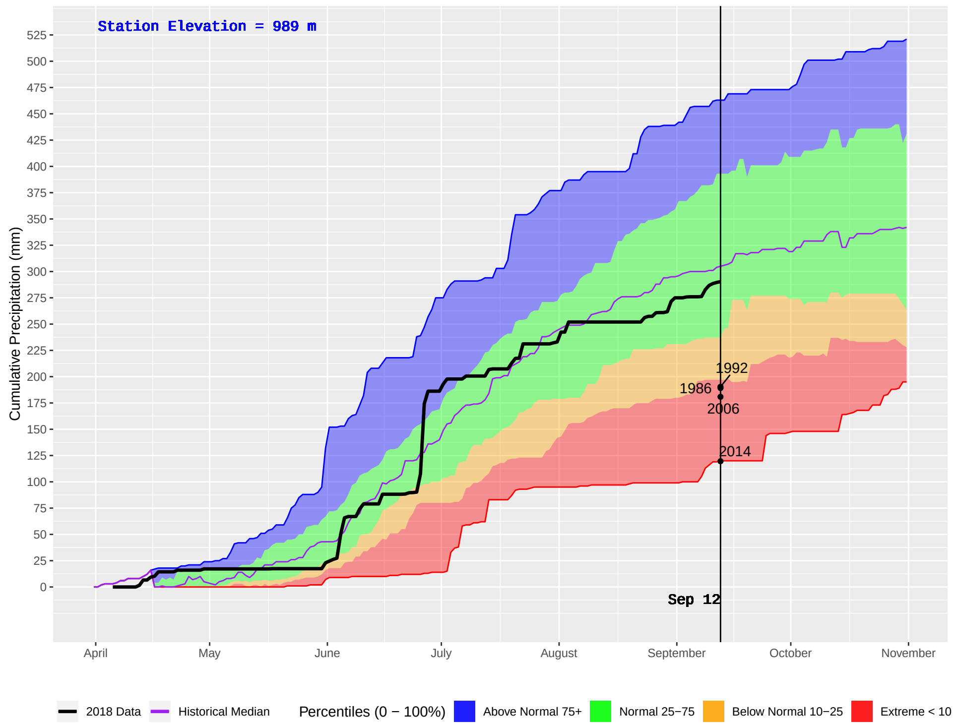
PINK MOUNTAIN (129) : Historical (1983–2016) and Current (2018) Daily Cumulative Precipitation
