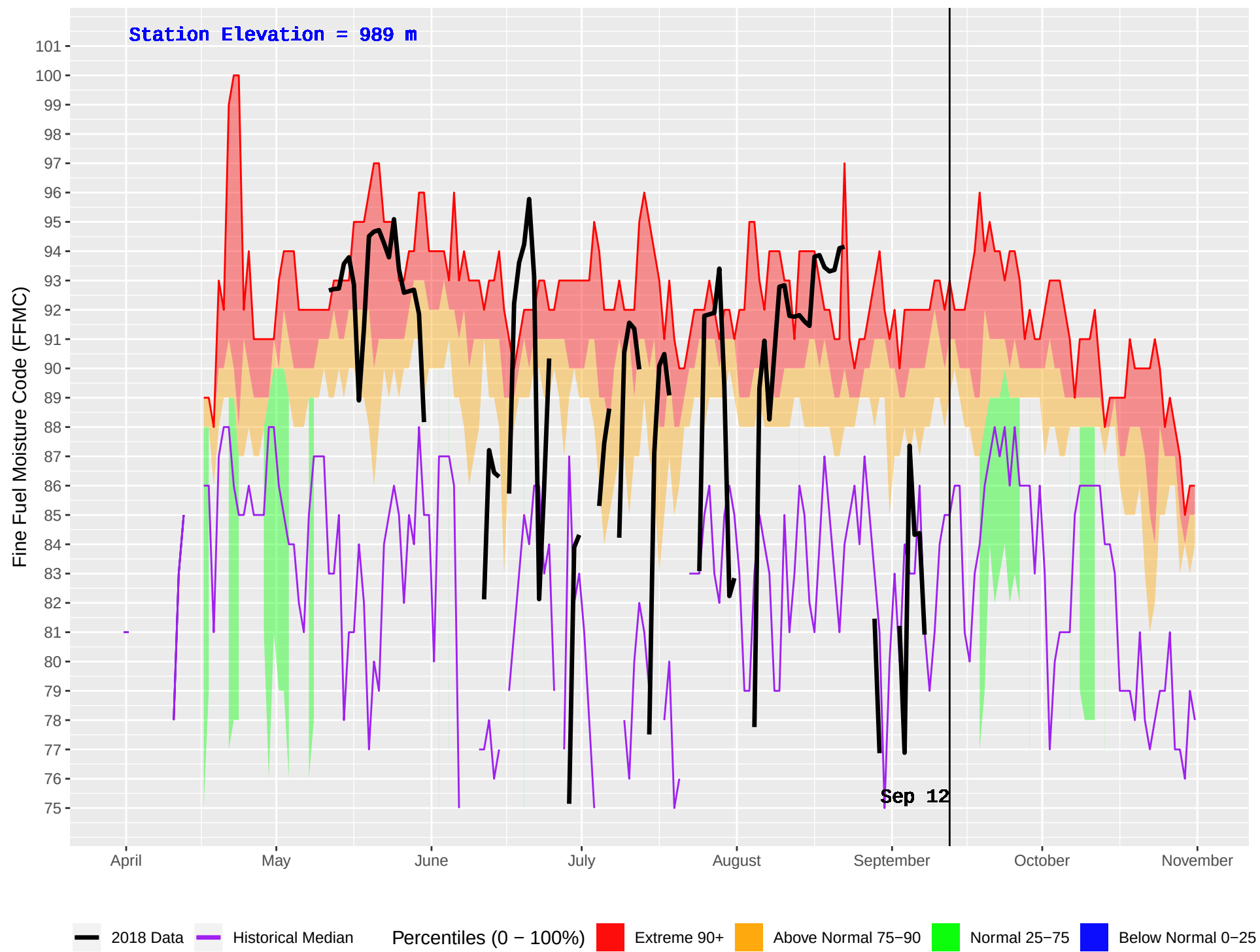
PINK MOUNTAIN (129) : Historical (1983–2016) and Current (2018) Daily Fine Fuel Moisture Code (FFMC)
